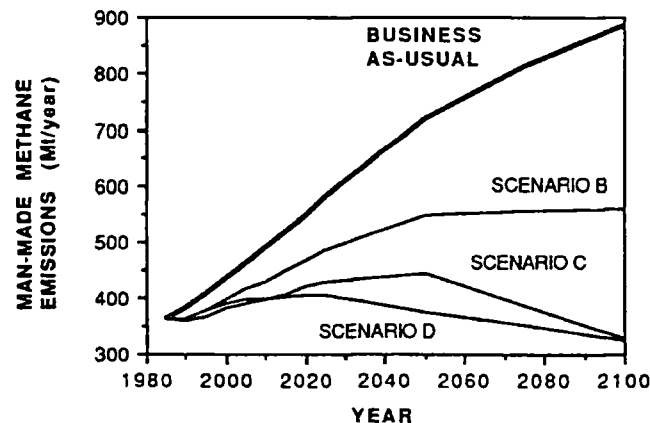
Figure 2 Projected man-made Methane emissions (Million tonnes per year)
